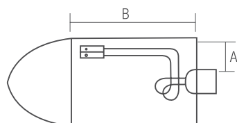
OUTBOARD Typical Outboard Cable Routing : A+B+3'=L
