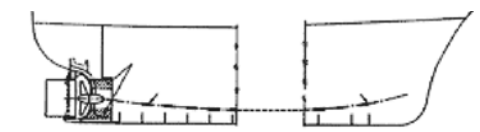
Typical galvanic anode for cathodic protection of a ship's hull (anodes alongside the hull are normally mounted alternately on both sides of dilge keels)
